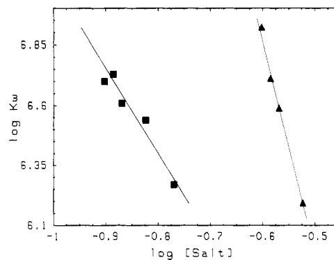
FIGURE 5: Effect of salt concentration on the affinity of recA protein for single-stranded DNA in the presence of CaCl 2 . The units of K\omega and salt concentration are M -1 and M, respectively. Protein titrations were conducted as described under Materials and Methods. The concentration of etheno M13 DNA was 1.57 μM. Experiments contained recA protein in 4 mM CaCl 2 at 37 °C using NaCl to vary the salt concentration: (▲) no cofactor ( y = -9.0x + 1.47 ); (■) 500 μM ADP ( y = -3.3x + 3.76 ).
