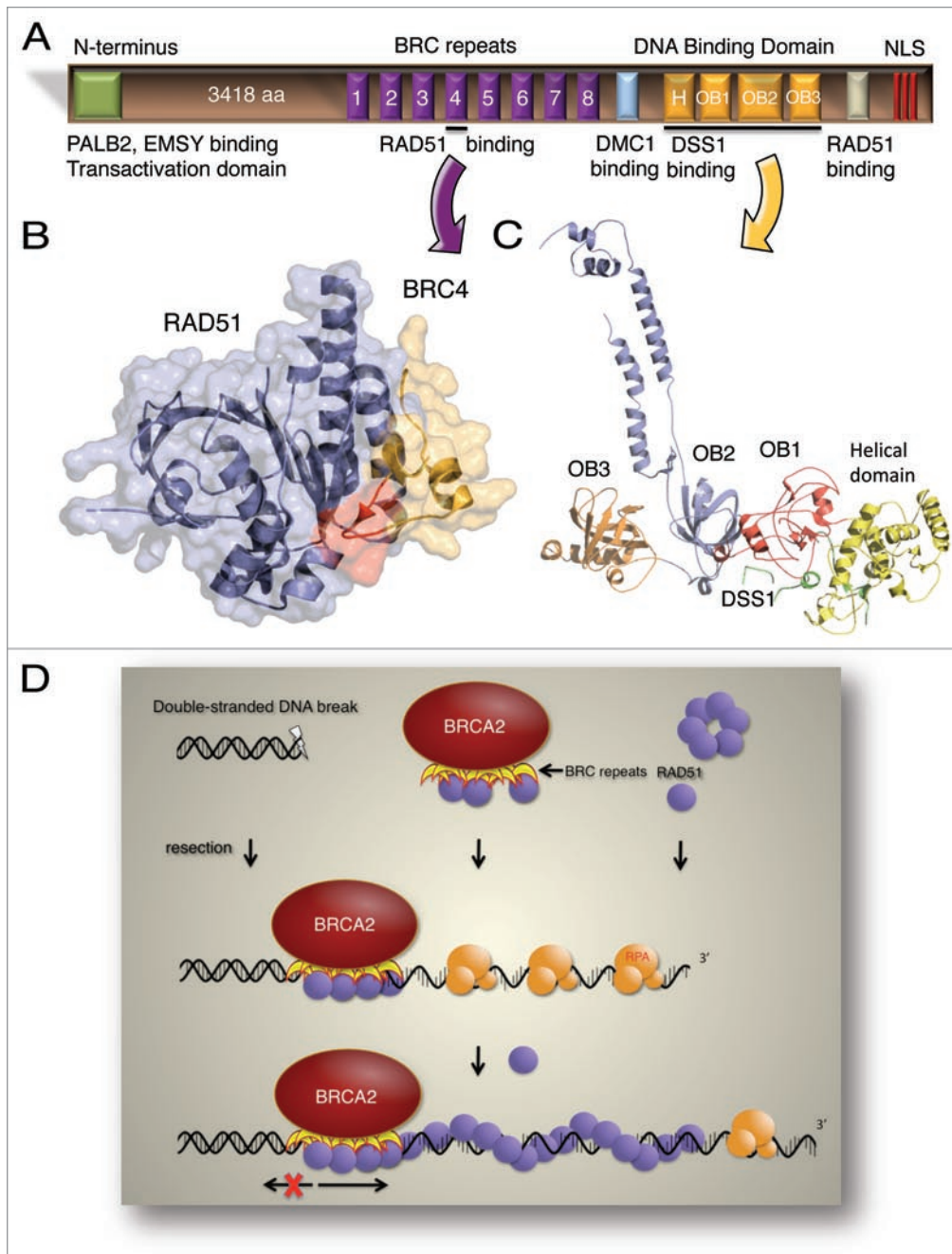
Figure 1. (A) Schematic representation of BRCA2 protein showing its functional domains. H, helical domain; OB, oligonucleotide-binding fold; NLS, nuclear localization signal. (B) Molecular surface and ribbon representation of RAD51 bound to BRC4 (PDB code 1n0w). RAD51 is shown in blue and BRC4 in orange. The highly conserved interacting region of BRC4 is highlighted in red. (C) Illustration of the DNA binding domain structure of mouse BRCA2 DBD-DSS1 (PDB code 1MIU). The helical domain is shown in yellow, and OB 1, 2 and 3 are shown in red, blue and orange, respectively. DSS1 protein is shown in green. (D) Model for the function of BRCA2 in the repair of DNA breaks. Through its DNA binding domain, BRCA2 targets RAD51 to the dsDNA-ssDNA junction of a resected DSB. Using its BRC repeats, BRCA2 directs RAD51 onto the ssDNA and blocks assembly onto dsDNA. This interaction likely provides a nucleus for nascent ATP-RAD51 filament formation. Subsequent growth of the nucleoprotein filament from this nucleus will displace RPA. Eventually, the RAD51-ssDNA filament will pair with an intact copy of the chromosome to continue the steps of DNA repair (not shown).
